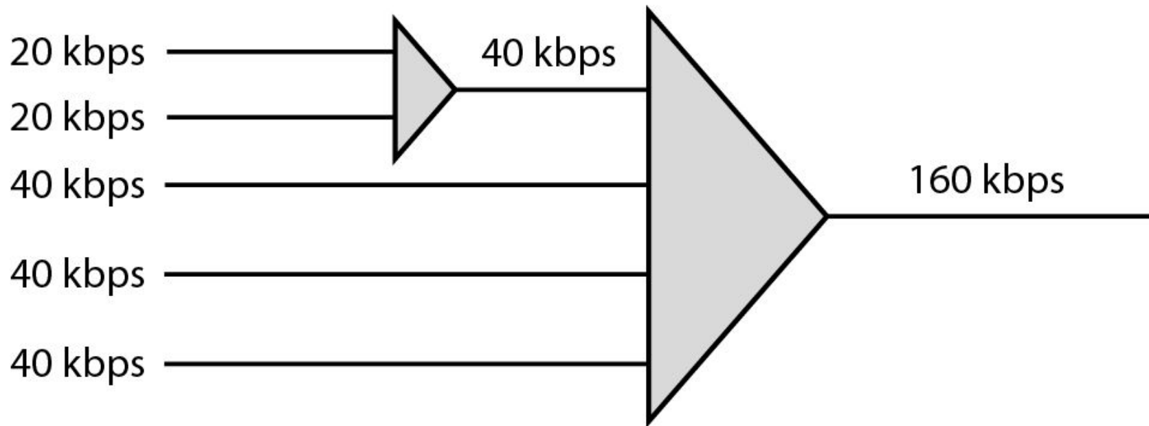
Figure 6.19 Multilevel multiplexing
